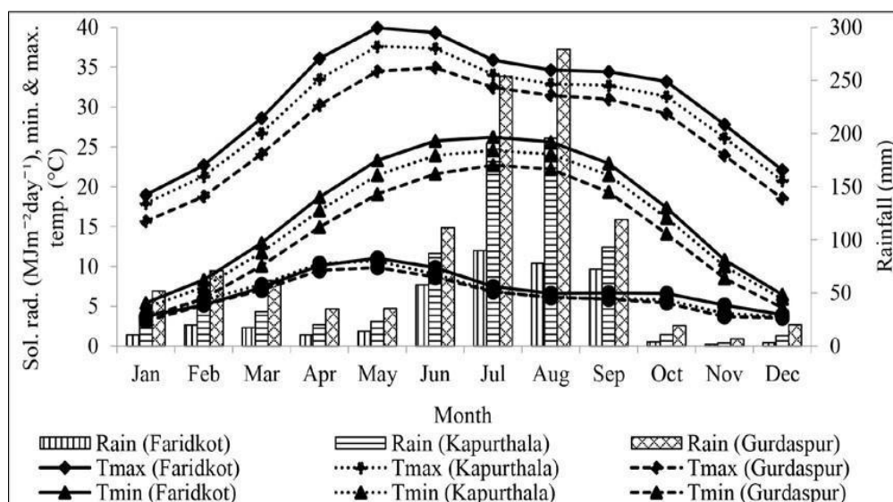
Figure 6: Monthly weather conditions at different locations in India during 2000-2017
