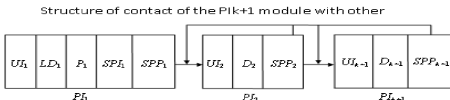
Figure1. Structure of the program of sorting
